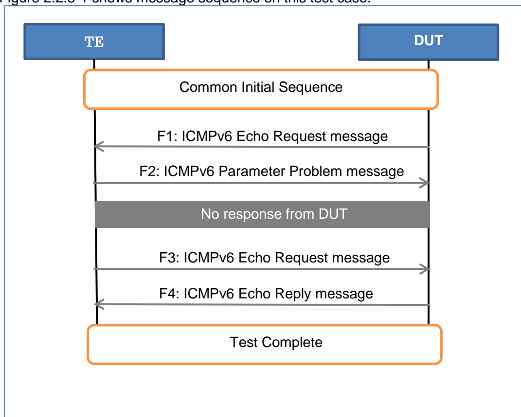
Figure 2.2.5-1 Message Sequence on Reception of ICMPv6 Parameter Problem message
